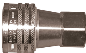
1367771 QUICK RELEASE COUPLER G3/4"(F) 16 MPA
