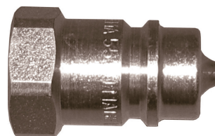
1367772 QUICK RELEASE NIPPLE G3/4"(F) 16 MPA
