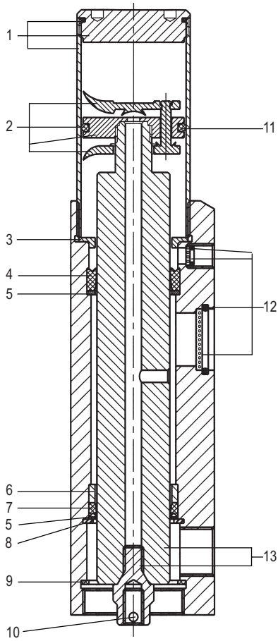
Air motor/luftmotor A11740-10 & A11741-10
