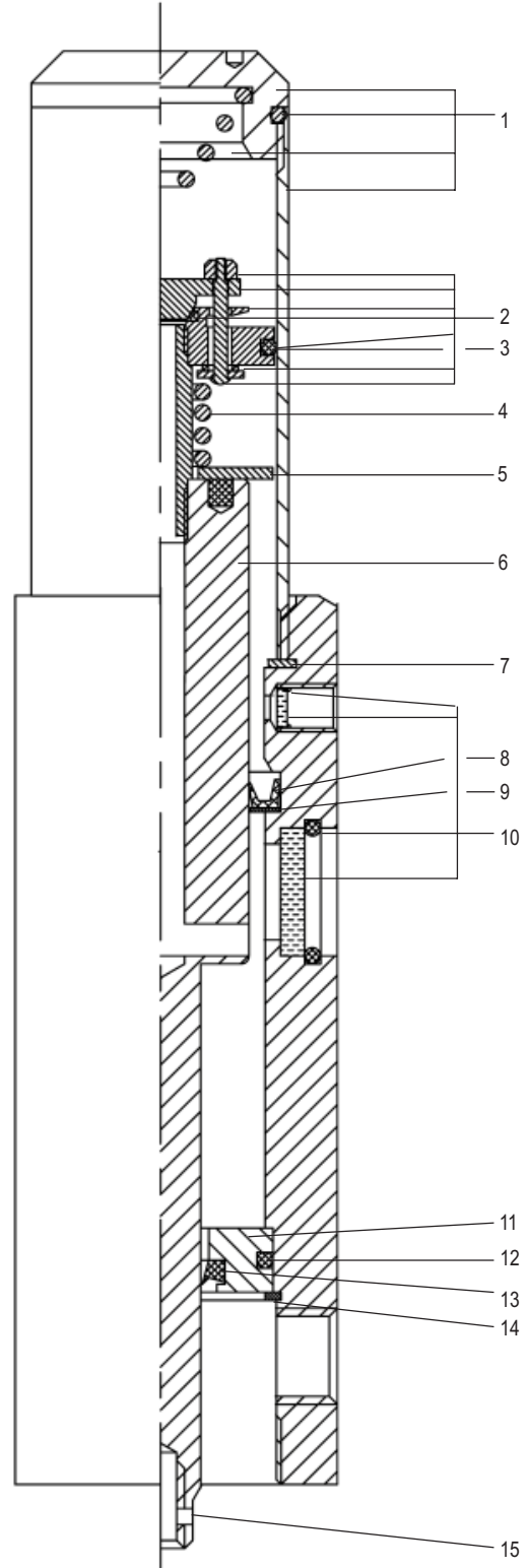
Air motor/luftmotor A15780-81
