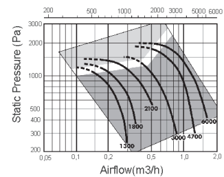
Pressure Drop Chart / Tryckfallstabell
