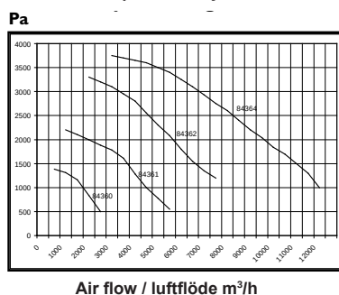
Pressure Drop Chart / Tryckfallstabell
